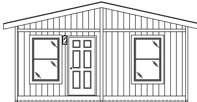
FRONT ENDWALL
